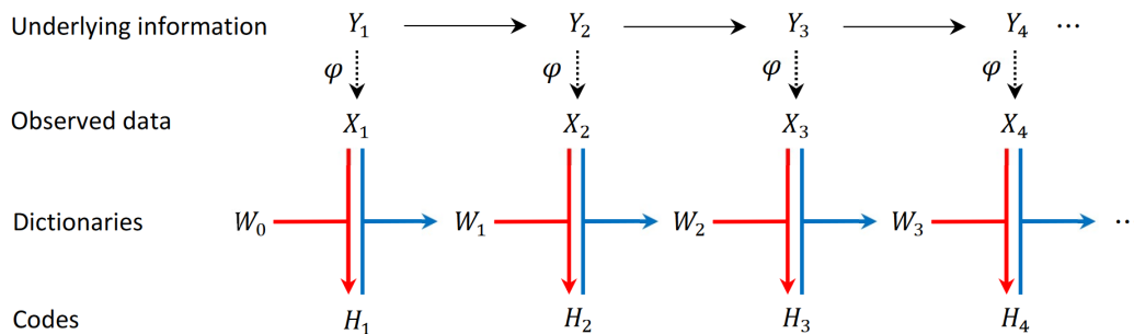
Figure 2: Iterative block scheme of functional OMF. (Y_t)_{t \in \mathbb{N}} is the sequence of underlying information. At each time t , a data matrix X_t of interest is observed from information Y_t via a fixed function \varphi . Sequences of dictionaries (W_t)_{t \in \mathbb{N}} and codes (H_t)_{t \in \mathbb{N}} are learned from data matrices by a block optimization scheme.
