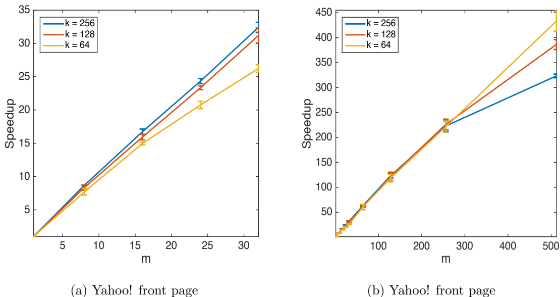
Figure 8: Running time of GREEDI compared to the centralized greedy algorithm. a) shows the ratio of centralized vs. distributed solution with k = 64, 128, 256 and up to m = 32 machines for Yahoo! Webscope data. b) shows the same ratio with k = 64, 128, 256 and up to m = 512 machines on the same dataset. Both experiments are performed on a cluster of 8 quad core machines.
