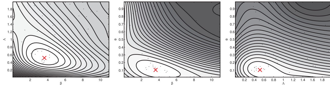
(b) 100 data points, \hat{\theta}_J^{(100)} = (3.61, 0.52, 0.11)
