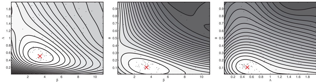
(c) 150 data points, \hat{\theta}_J^{(150)} = (3.43, 0.50, 0.10)
