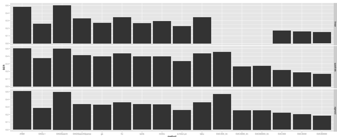
Figure 3: Balanced Error Rate of the different methods for small size DAGs and three types of dependency (top: linear, middle: quadratic, bottom: sigmoid). The notation D2Cx stands for D2C with a training set of size x and where training and test sets are based on DAGs with the same type of dependency. The notation D2Cx.lin stands for D2C with a training set of size x based on DAGs with linear dependency only.
