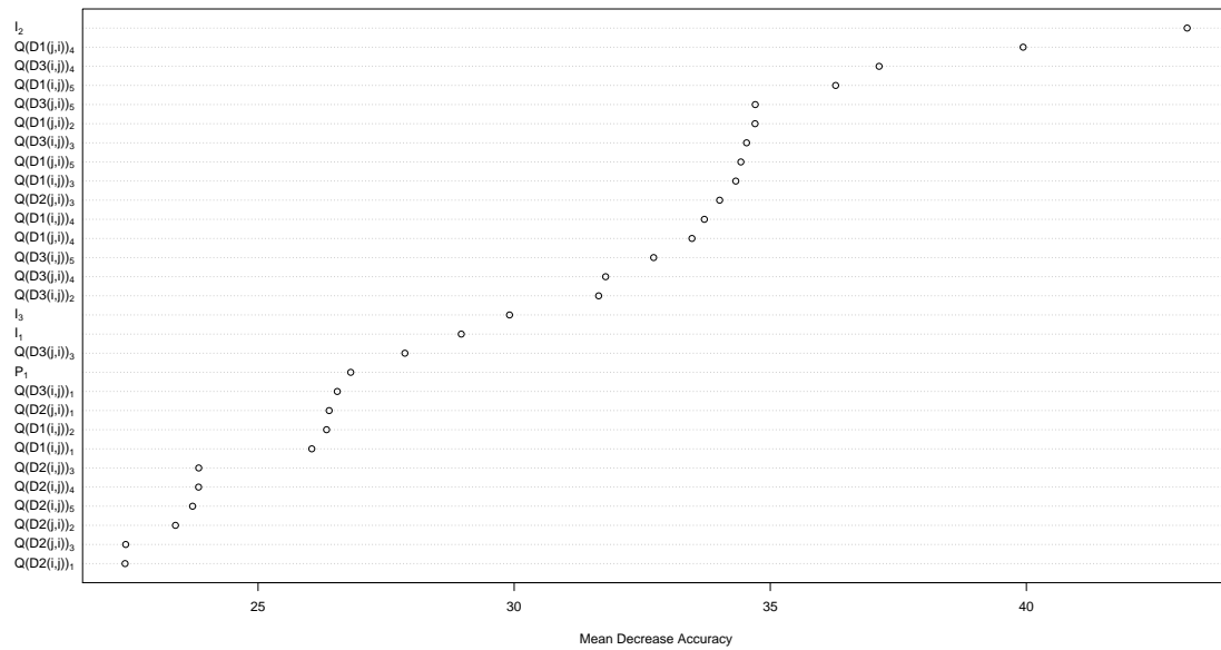
Figure 2: Importance of D2C features returned by the Random Forest mean decrease accuracy. I_i denotes the i th component of the descriptor vector (18) while Q(Dx(i, j))_k denotes the k th quantile of the population of descriptor Dx(i, j) .
