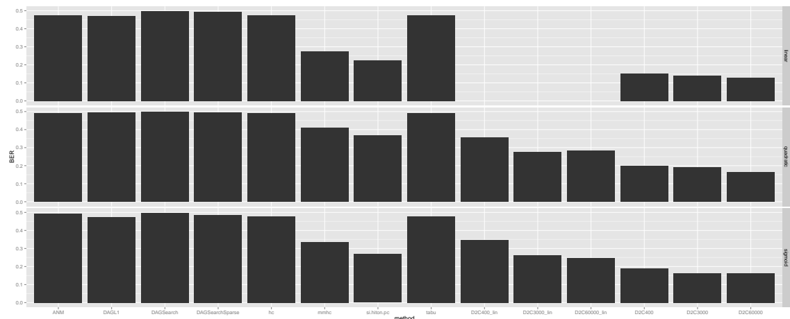
Figure 5: Balanced Error Rate of the different methods for large size DAGs and three types of dependency (top: linear, middle: quadratic, bottom: sigmoid). The notation D2Cx stands for D2C with a training set of size x and where training and test sets are based on DAGs with the same type of dependency. The notation D2Cx_lin stands for D2C with a training set of size x based on DAGs with linear dependency only.
