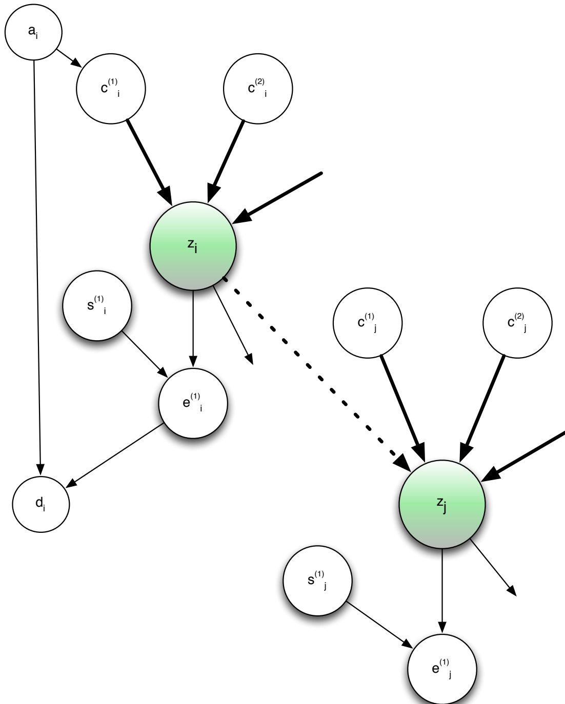
Figure 1: Two causally connected variables and their Markov Blankets.
